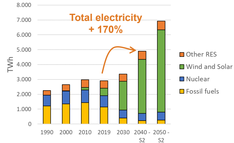
Electricity generation by energy vector
