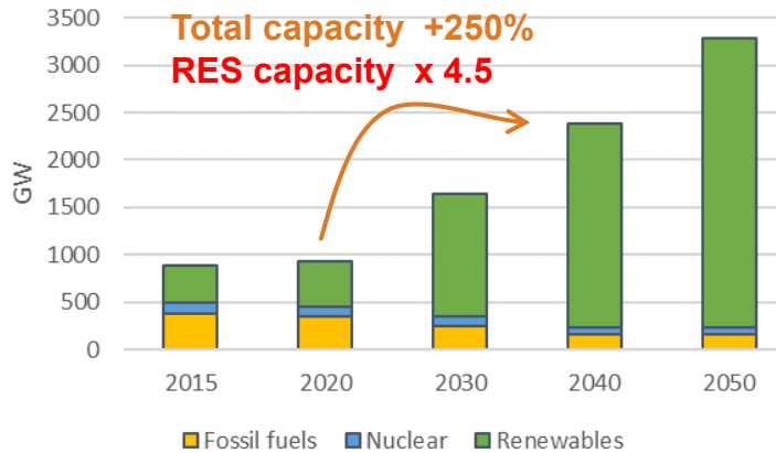
Net installed capacity by energy carrier (Sc. 2)
