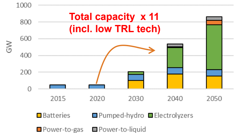
Net installed storage and new fuels production capacity (Sc. 2)
